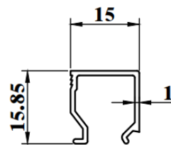
SWD344 WEIGHT : 0.139 KG/M AP : 100.52mm
