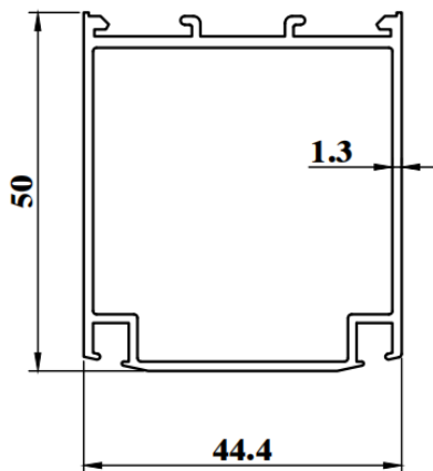
SWD341 WEIGHT : 0.763 KG/M AP : 241.74mm
