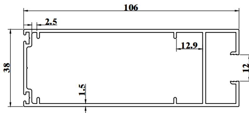
SWD351K WEIGHT : 1.324 KG/M AP : 397.54mm
