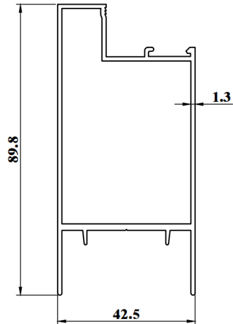
SWD340 WEIGHT : 1.048 KG/M AP : 336.94mm
